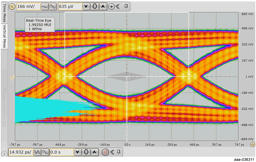
Fig. 7. HDMI 2.1 12G FRL eye diagram, PCB with device; typical values
